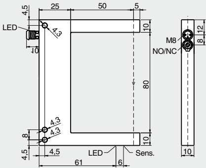
Rotlichtvariante anreihbar Red light version mountable side by side
